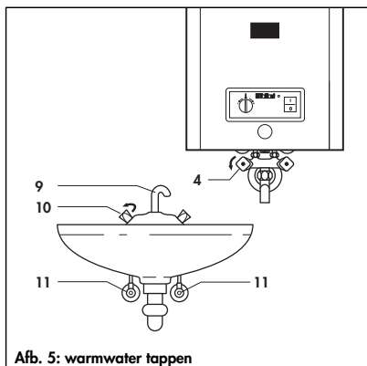
Afb. 5: warmwater tappen
